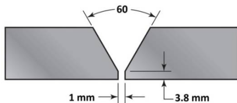
Single-V Groove Weld
